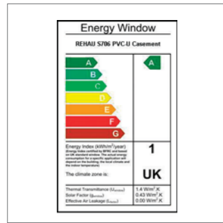
Chart shows Window Energy Rating for REHAU Tritec windows.
